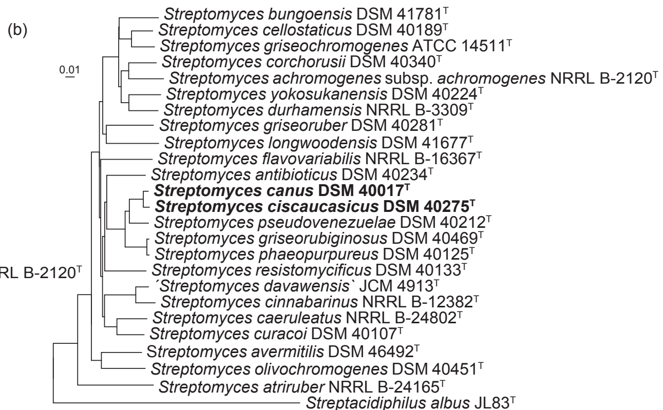
Core genome (amino acid sequence)
