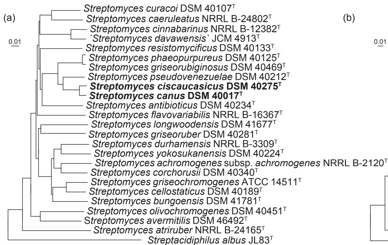
Core genome (nucleotide sequence)
